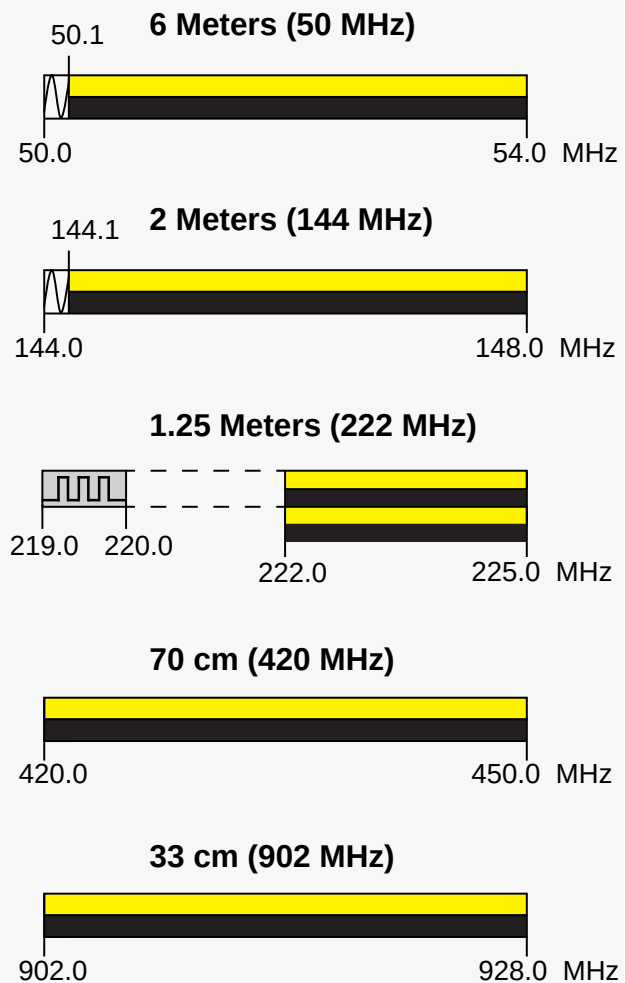
Figure 2.3. Radio Signal Wavelengths
