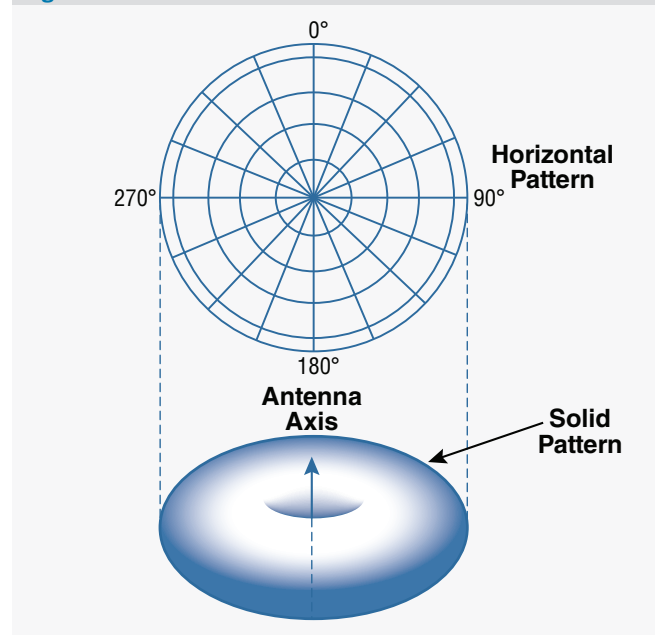
Figure 2.13. Omnidirectional Antenna Pattern
